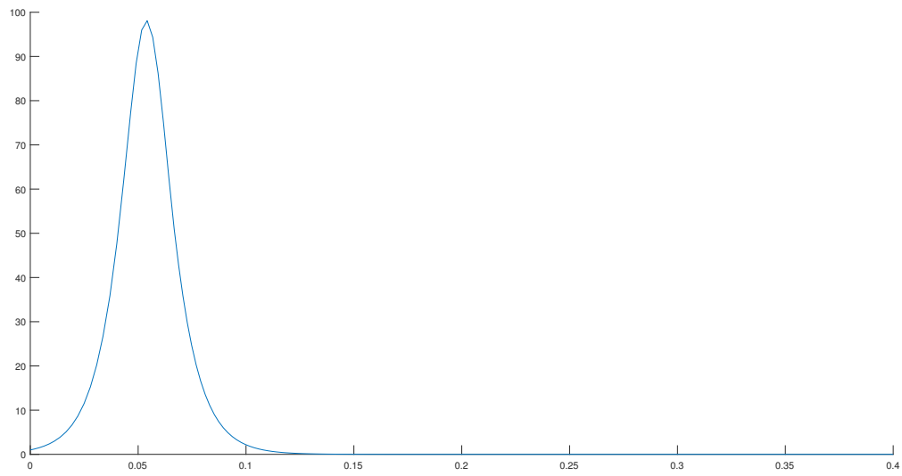
Figure 1: Simulation of behavior of x
