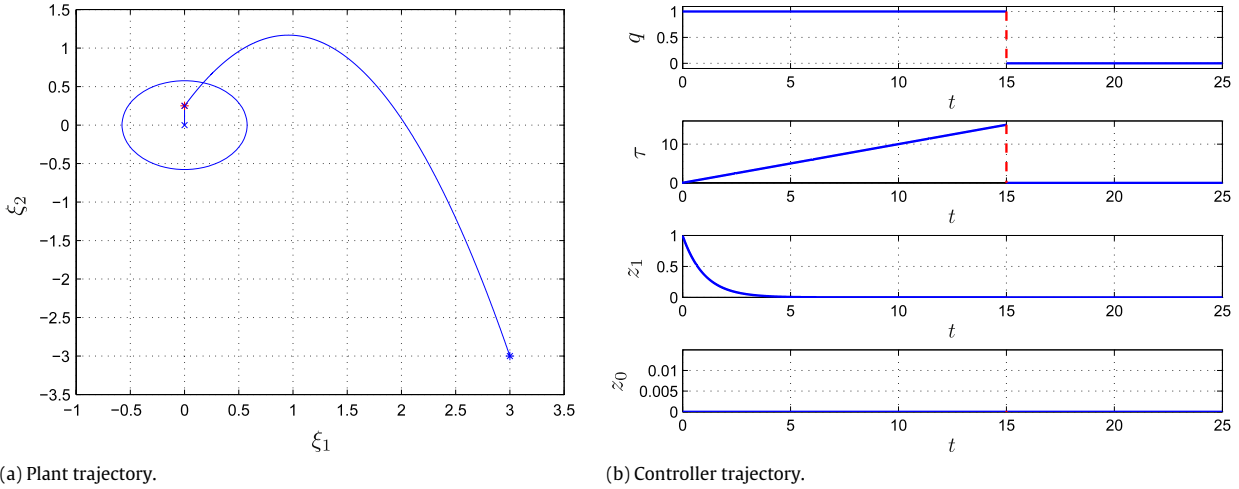
Fig. 4. Plant and controller states of a closed-loop trajectory. (a) Plant component \xi(t, j) for (13) from \xi(0, 0) = (3, -3) , q(0, 0) = 1 , \tau(0, 0) = z_0(0, 0) = 0 , z_1(0, 0) = 1 . Dotted lines denote an estimate of \mathcal{B}_0 , \star (red) the jump from q = 1 to 0, and \times the sets \mathcal{A}_1 = (0, \bar{\alpha}) and \mathcal{A}_0 = (0, 0) , with \bar{\alpha} = \frac{1}{4} . (b) Controller states of hybrid supervisor \mathcal{K}_s . The dashed lines represent the jumps in the variables. Controller parameters: \varepsilon_{0,a} = \frac{4}{27} , \varepsilon_{1,a} = 0.00005 , and \tau^* = 15 . (For interpretation of the references to colour in this figure legend, the reader is referred to the web version of this article.)
