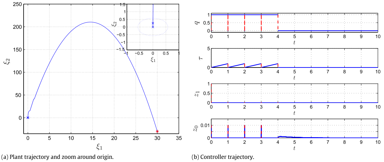
Fig. 3. Plant and controller states of a closed-loop trajectory. (a) Plant component \xi(t, j) for (13) from \xi(0, 0) = (30, -30) , q(0, 0) = \tau(0, 0) = z_0(0, 0) = 0 , z_1(0, 0) = 1 . Dotted lines denote an estimate of \mathcal{B}_0 , \star (red) the jump from q = 1 to 0, and \times the sets \mathcal{A}_1 = (0, \bar{\alpha}) and \mathcal{A}_0 = (0, 0) ( = \mathcal{A} ), with \bar{\alpha} = \frac{1}{4} . (b) Controller states of hybrid supervisor \mathcal{K}_s . The dashed lines represent the jumps in the variables. Controller parameters: \varepsilon_{0,a} = \varepsilon_{1,a} = 0.01 , and \tau^* = 1 . (For interpretation of the references to colour in this figure legend, the reader is referred to the web version of this article.)
