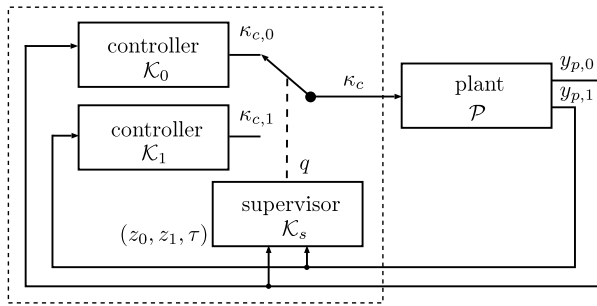
Fig. 1. Proposed control approach for Problem ( \star ).
