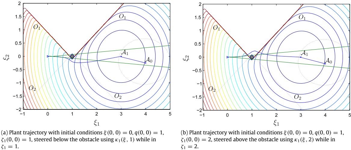
Fig. 5. Trajectories \xi(t, j) to the point-mass system with hybrid supervisor \mathcal{K}_s . Dotted circle denotes an estimate of \mathcal{B}_0 and \times the sets \mathcal{A}_1 = \{(3, 0)\} and \mathcal{A}_0 = \{(4, -\frac{1}{4})\} . The set O_1 is the region below the upper “wedge,” while the set O_2 is the region above the lower “wedge”, which is depicted in dotted line. The cone emanating from the initial condition depicts that, initially, the target point is not in the line-of-sight of the point-mass system. The controller parameters used are \mu = 1.1 and \lambda = 0.09 .
