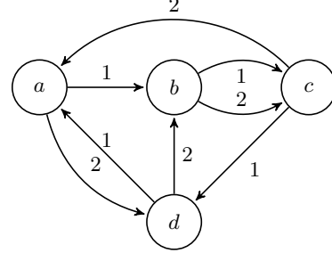
Figure 9: A graph \mathbf{G} whose feasibility implies that of \mathbf{G}^* (Example 4).
