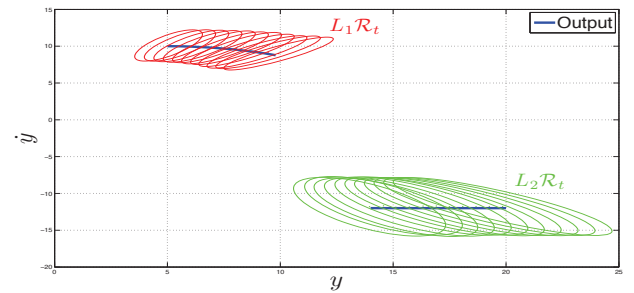
Fig. 2. The sets \mathcal{Z}_1(t) , \mathcal{Z}_2(t) , and the output trajectory in (y, \dot{y}) space.
