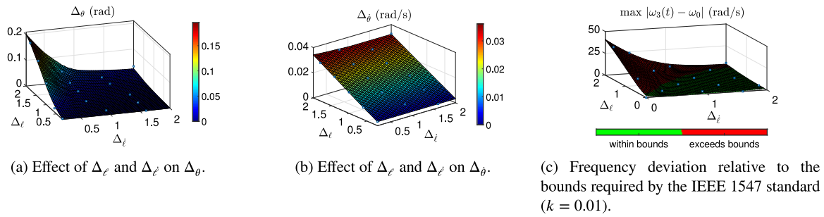
Fig. 2. Effects of load change on control performance.
